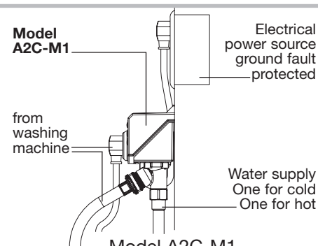
Model A2C-M1
